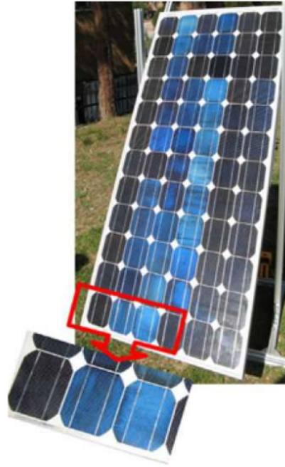
FIGURE 5. Decolouring of cells due to a change in ARC [10]
