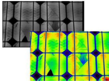
FIGURE 1. Cracks in the cell [10]
