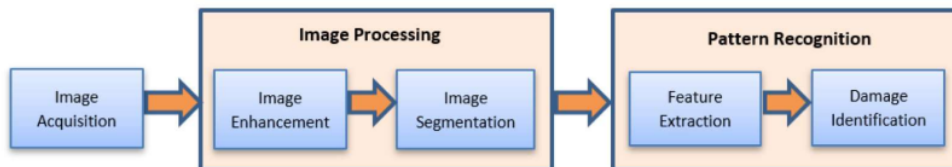
FIGURE 9. Common process of computer vision techniques for damage detection
