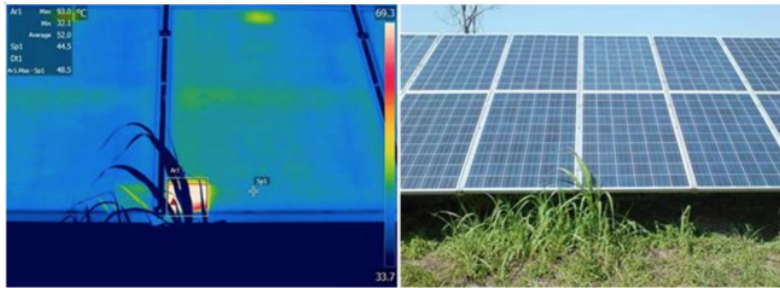
FIGURE 8. PV module shows overheated cells due to shading by plants [13].
