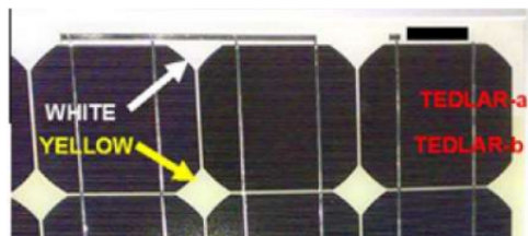
FIGURE 3. Discoloration of a PV module
