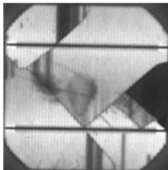
FIGURE 7. EL image of a solar cell with a typical crack pattern [13]
